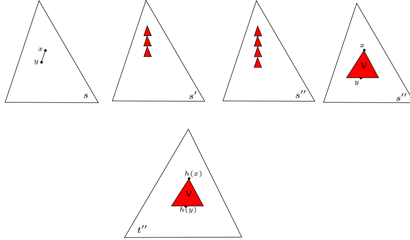
Fig. 4. This figure depicts the last step of the proof. The top left tree is s , which is k -pseudo-included in t'' depicted at the bottom. The extra part of t'' \setminus h(s) is depicted in dark grey and is the abstract context V . The second tree in the top row represents s' after applying Lemma 4, the dark grey parts representing U = V^{l'} . Aperiodicity adds one more copy of V and yields the third tree in the top row. But this tree is essentially the initial one with V added between x and y , as depicted by the top right tree.
