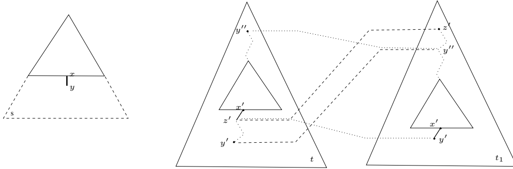
Fig. 3. Illustration of the first case. s is depicted on the left, with U the solid triangle within it. t is in the middle, with the weak pseudo-image of U depicted as a solid triangle within it. The tree t_1 resulting from the swap is shown on the right. Notice that y' becomes a child of x' and that no other nodes of the weak pseudo-inclusion are affected.
