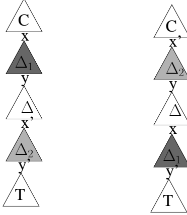
Fig. 1. Illustration of the vertical swap
