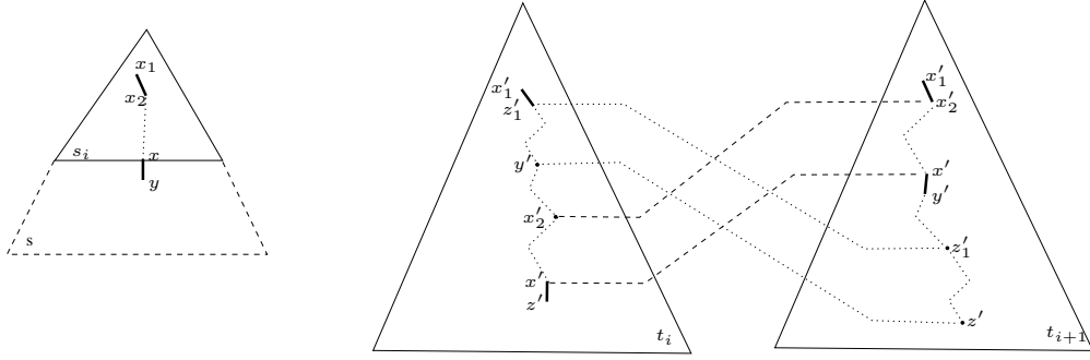
Fig. 2. This illustrates the case when x' is a descendant of x'_2 . s_i and s are depicted on the left. t_i is depicted in the middle. After applying the k -guarded vertical swap between [z'_1, y'] and [x'_2, z'] , we reach t_{i+1} depicted to the right. The nodes z'_1 and x'_2 have the same k -types and the nodes y' and z' have the same k -types.
